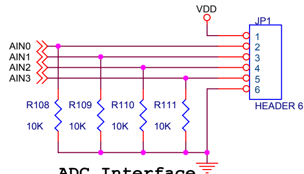
ADC Interface
