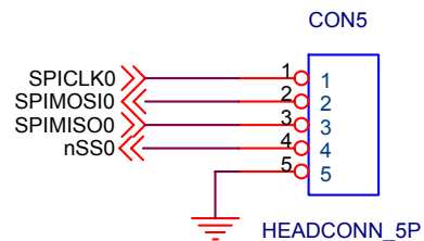
SPI Interface
