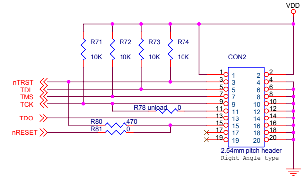
JTAG/Multi-ICE Connector
