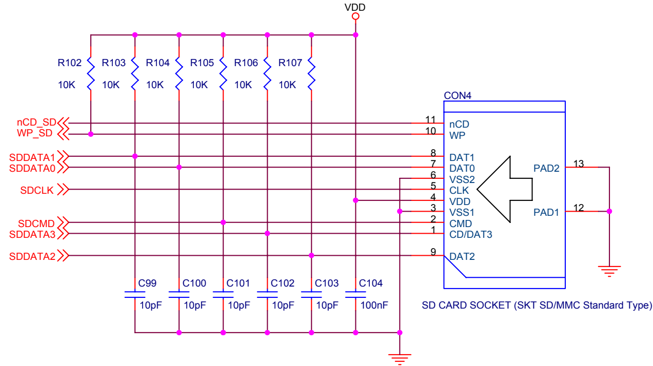
SD CARD
